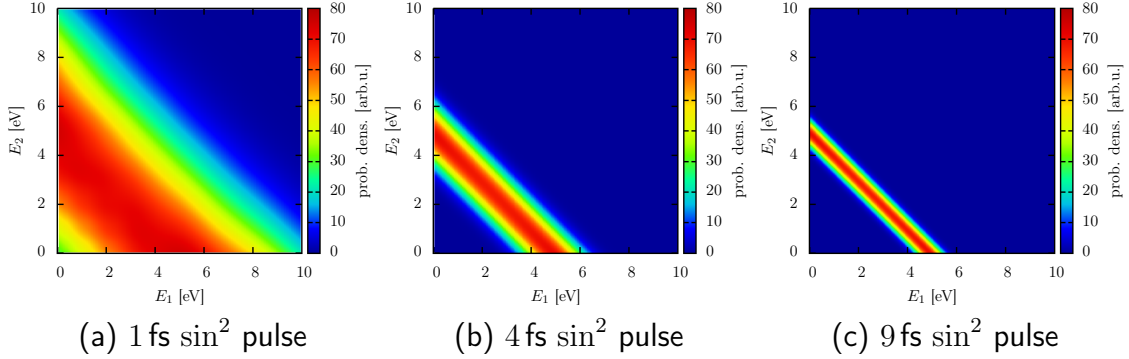
Figure 9.1: Energy distribution after two-photon double ionization from three different laser pulses with a mean energy of \langle \omega \rangle = 42 eV. All three pulses have a \sin^2 envelope for the vector potential, with total durations (a) 1 fs ( \sim 10 cycles), (b) 4 fs ( \sim 40 cycles), (c) 9 fs ( \sim 90 cycles). The distributions are centered around the line E_1 + E_2 = 2\langle \omega \rangle - I_1 - I_2 \approx 5 eV. The width of the distribution directly shows the energy uncertainty due to Fourier broadening.
