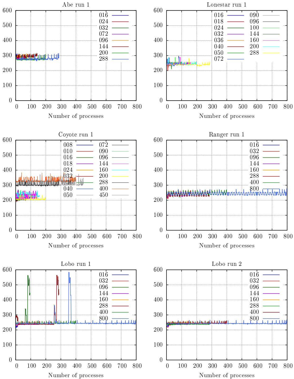
Figure D.1: Runtimes in seconds for the single electron Hamiltonian operator.
