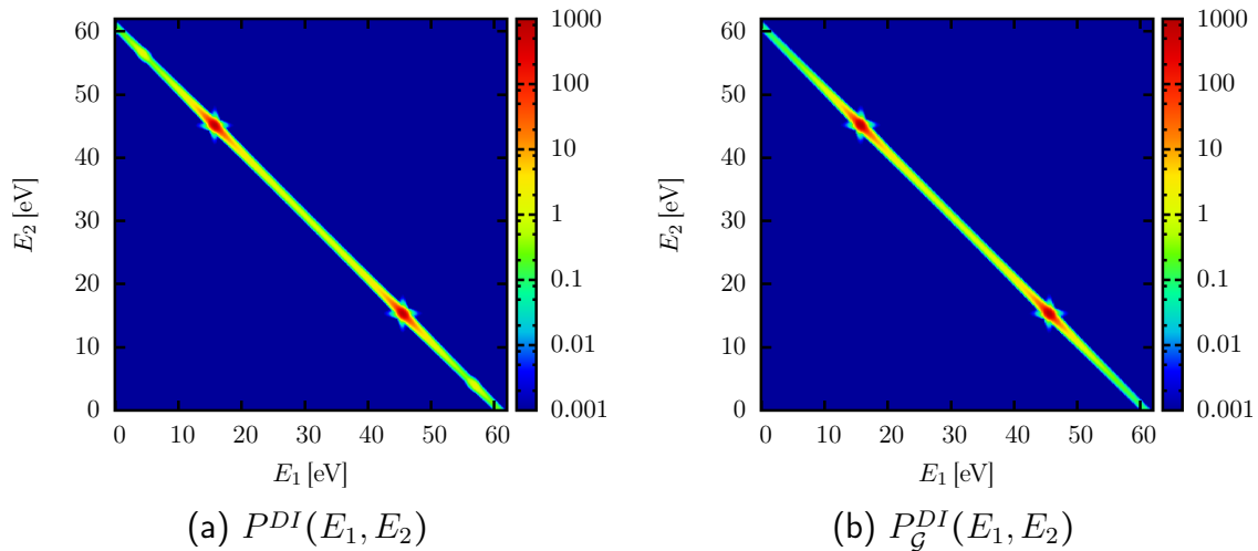
Figure 11.2: Energy distribution for TPDI from a 9 fs \sin^2 pulse at \hbar\omega = 70 eV. (a) shows the distribution obtained from the full solution of the TDSE, (b) shows the strongly simplified model P_G^{DI} . The agreement is remarkably good.
