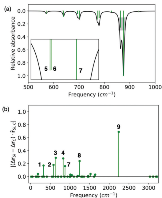
Fig. 3 (a) Calculated IR spectrum of R I at the B3LYP/6-31+G(d,p) level in methanol (inset highlighted in grey). (b) Relative normalized Cartesian displacements ( \Delta r in the text) between the silicon and sp carbon atoms in R I along the Si–C(sp) bond axis.
