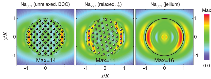
Figure 5: Contour plots of the EFE for the BCC \text{Na}_{331} , ICO \text{Na}_{297} , and jellium \text{Na}_{331} clusters at the corresponding Mie LSP resonance. The E -field amplitudes are normalized to their maximum value, which is indicated in each panel. The incident E -field is directed along the X axis.
